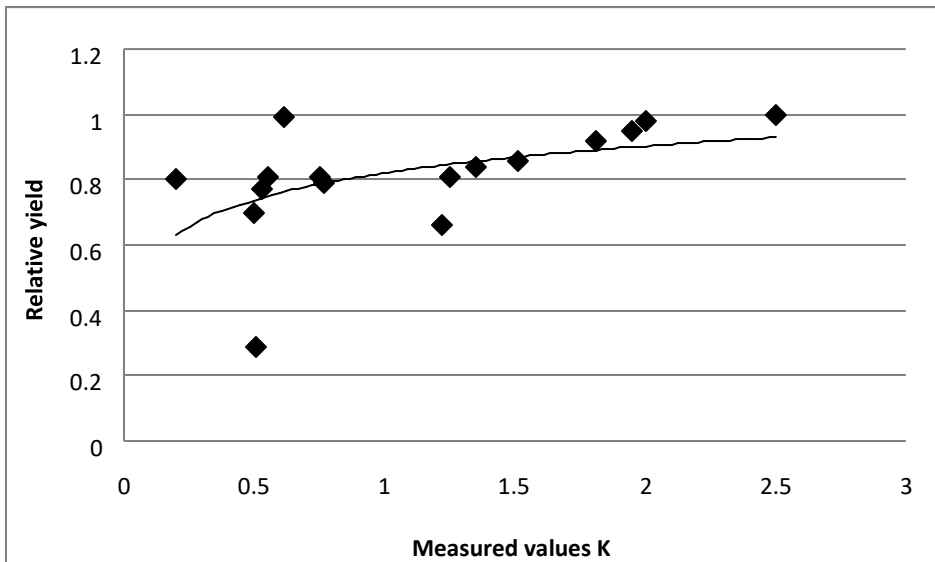
Figure 4: Functional relationships between potassium and relative yield of maize after Aune and Lal (1997)
