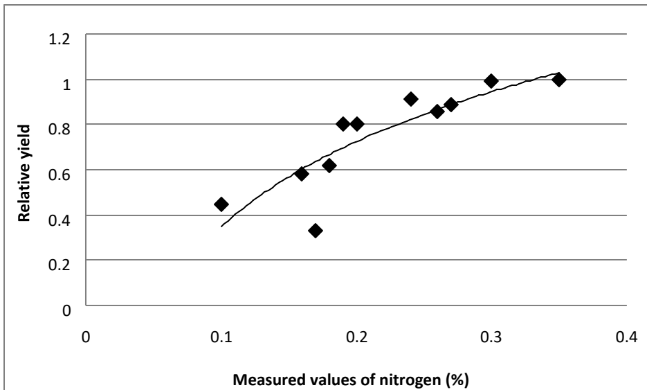
Figure 2: Functional relationships between nitrogen and relative yield of maize after Aune and Lal (1997)
